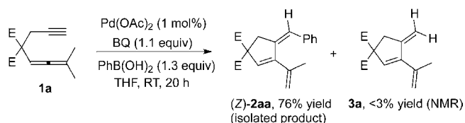
Scheme 2. Oxidative phenylating carbocyclization of allenyne 1a . E = CO 2 Me.
